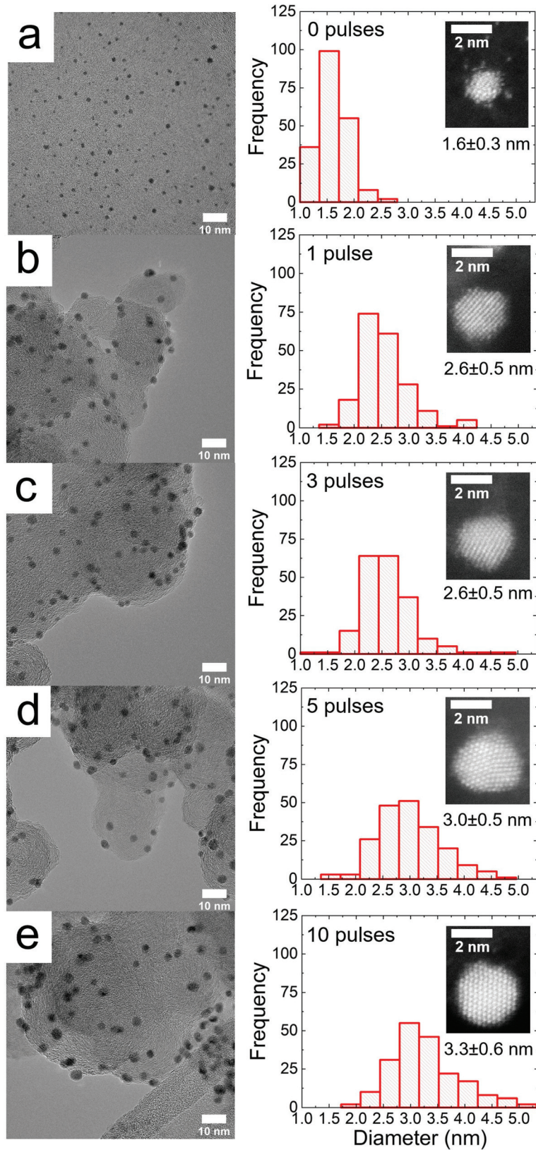
Fig. 1 TEM micrographs and the associated size-distribution histograms for HT Pt electrodeposition onto Au 147 DENs using the indicated number of pulses. Each histogram was obtained by sizing 200 randomly selected NPs. Aberration-corrected STEM (acSTEM) micrographs of representative particles are shown in the insets of the histograms.
