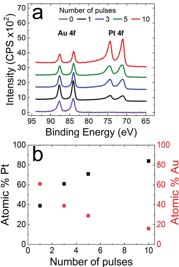
Fig. 3 (a) XPS spectra in the Au 4f and Pt 4f regions for HT Pt electrodeposition onto the Au 147 DENs using the indicated number of pulses. (b) Au and Pt atomic compositions as a function of pulse number. The data were obtained by integrating the peaks in (a).
