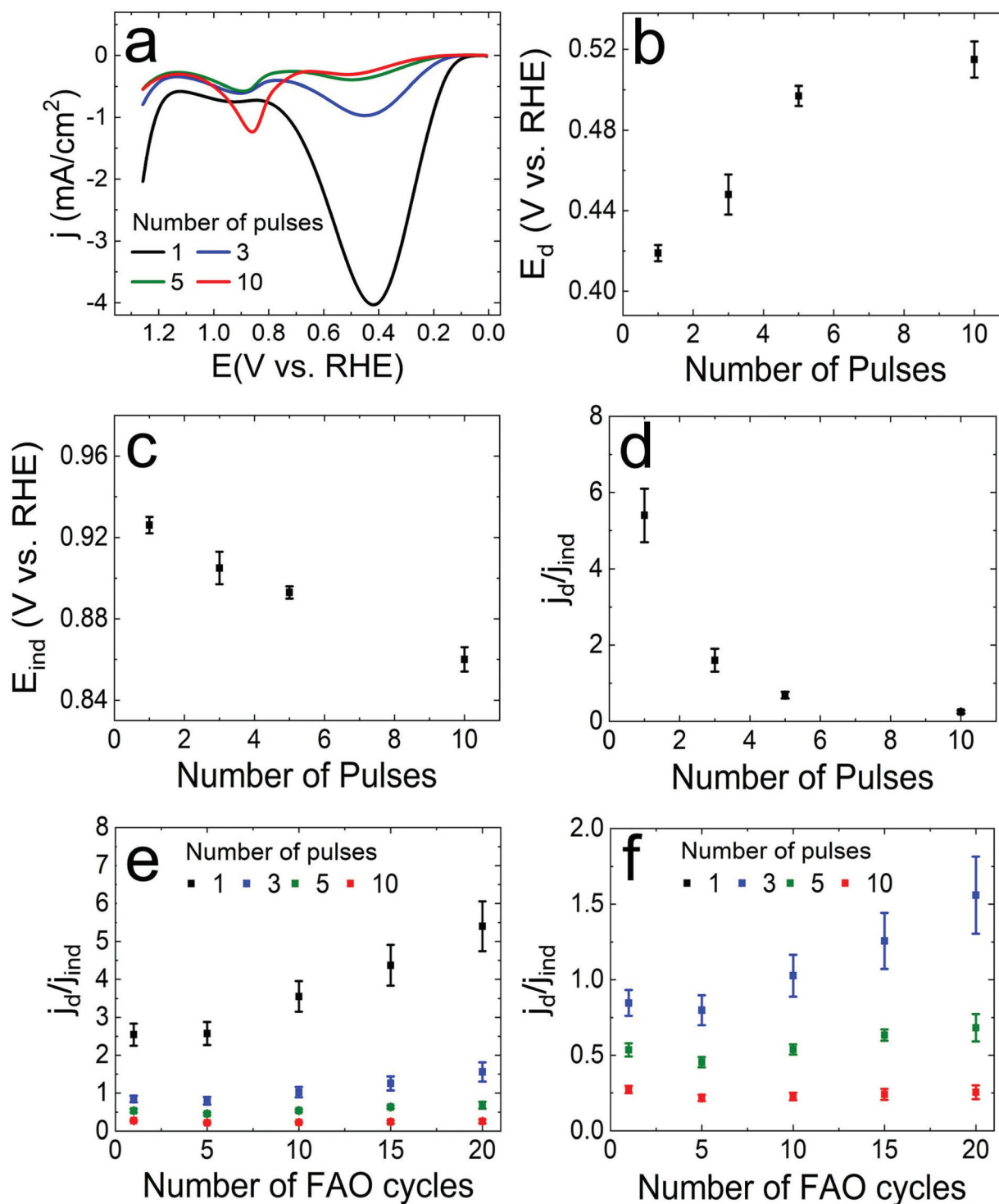
Fig. 5 (a) FAO scans for the AuPt DENs synthesized via HT Pt electrodeposition onto Au 147 DENs as a function of pulse number. Just the forward-going scan of the 20 th FAO CV is shown. Peak positions for the (b) direct ( E_d ) and (c) indirect ( E_{ind} ) FAO pathways as a function of the number of HT Pt electrodeposition pulses. (d) The ratio of the current densities associated with the direct ( j_d ) and indirect ( j_{ind} ) FAO peaks. (e) The effects of FAO cycling on the j_d/j_{ind} ratios. (f) Expanded view of (e) for just 3 to 10 HT pulses. In all cases the electrolyte was N 2 -purged 0.50 M H 2 SO 4 containing 0.50 M formic acid. The scan rate was 10 mV s -1 .
