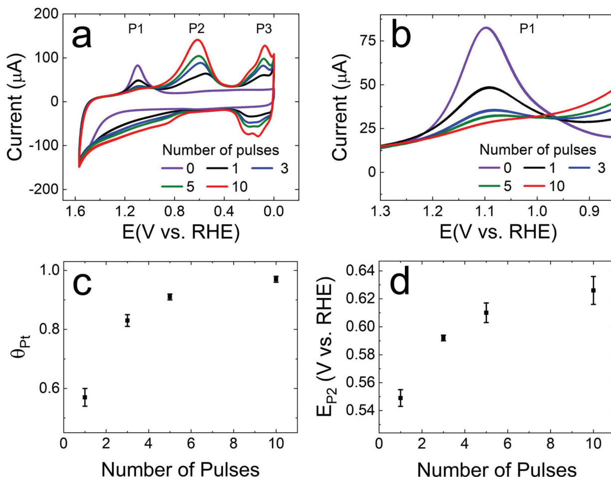
Fig. 2 (a) CVs recorded before and after HT Pt electrodeposition onto \text{Au}_{147} DENs using the indicated number of pulses. Peaks P1, P2, and P3 correspond to \text{AuO}_x reduction, \text{PtO}_x reduction, and Pt-H adsorption/desorption (Pt-hydride) peaks, respectively. (b) Expanded view of Peaks P1, showing that the \text{Au}_{147} NP surface is nearly completely covered after 3 to 5 HT pulses. (c) Pt coverage ( \theta_{\text{Pt}} ) as a function of pulse number. (d) The position of Peak P2 as a function of pulse number. The electrolyte was \text{N}_2 -purged 0.10 M \text{HClO}_4 and the scan rate was 100 \text{ mV s}^{-1} .
