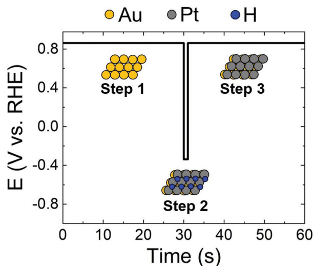
Scheme 1 Illustration showing the pulse sequence used for the HT method.
