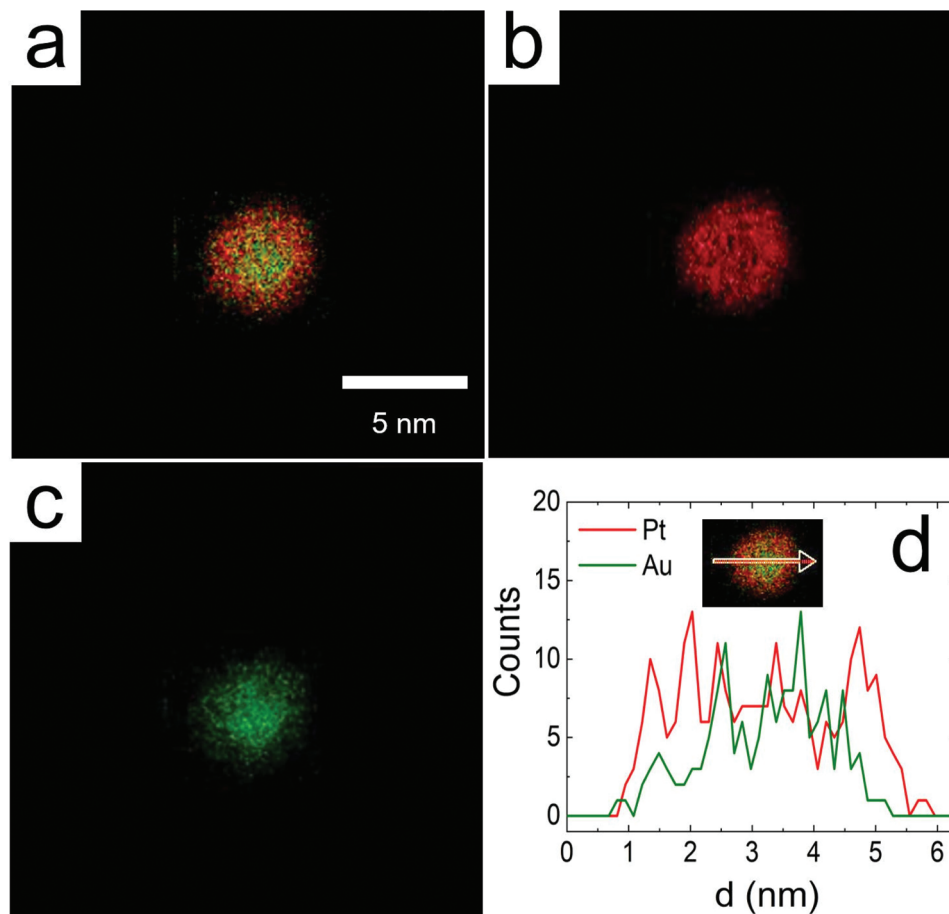
Fig. 4 Single-particle EDS maps for HT Pt electrodeposition onto Au 147 DENs using 10 pulses. (a) Superposition of the Pt and Au element maps. Pt and Au are shown in red and green, respectively. Individual element maps for (b) Pt and (c) Au. (d) Line profile extracted from the map in (a). The direction of the line scan along the associated map is shown in the inset and is indicated by the arrow. An additional, higher resolution line profile is provided in Fig. S4.† A core@shell structure is evident in both the maps and the line scans.
