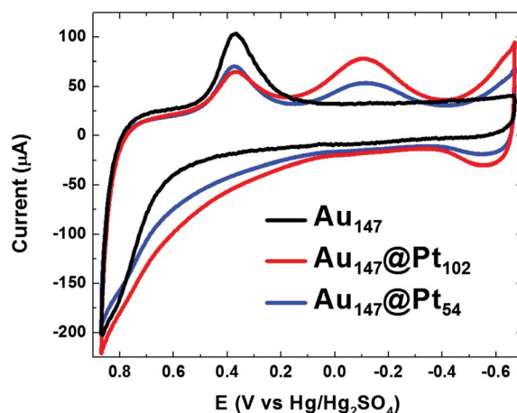
Fig. 1 CVs of the indicated DEN-modified glassy carbon electrodes (geometrical area = 0.247 cm 2 ). The scan rate was 100 mV s -1 and the aqueous electrolyte contained N 2 -saturated 0.10 M HClO 4 .
