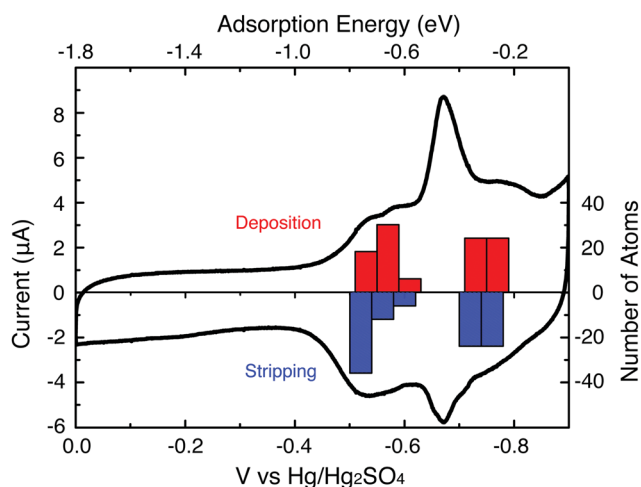
Fig. 2 A CV showing the Pb UPD process at a Au 147 DEN-modified glassy carbon electrode. The scan rate was 5 mV s -1 and the aqueous electrolyte solution contained 1.0 mM Pb(NO 3 ) 2 in 0.10 M HClO 4 . The DFT-calculated potentials for Pb deposition (red bars) and stripping (blue bars) are also shown.
