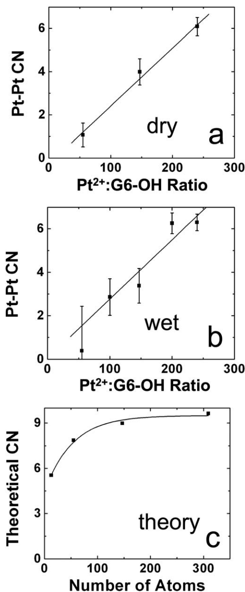
Fig. 4 Comparison of the Pt-Pt CNs for (a) dry and (b) wet Pt DENs at the indicated \text{Pt}^{2+} :G6-OH ratios. (c) Calculated M-M CNs for cuboctahedral particles in this size range. Reprinted with permission from ref. 72. Copyright 2008 American Chemical Society.
