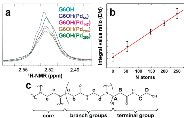
Figure 1. (a) Expansion of ^1\text{H} NMR region corresponding to the d proton resonances of \text{G6-OH}(\text{Pd}_n) . (b) I_D/I_d plotted versus the average number of atoms in each Pd DEN. (c) Schematic representation of \text{G6-OH} indicating the lettering scheme used to identify the methylene groups. 1 Numerical values corresponding to the data in this figure are provided in Table S1 (Supporting Information).
