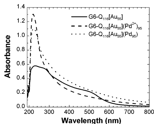
Figure 4. UV-vis spectra of G6-Q 116 [Au 55 ] seeds and G6-Q 116 [Au 55 ](Pd 95 ) core/shell DECS synthesized by the sequential-loading method before and after reduction using H 2 gas. The total metal concentration is 55 μM for the Au seeds and 150 μM for the G6-Q 116 [Au 55 ](Pd 95 ) solution.
