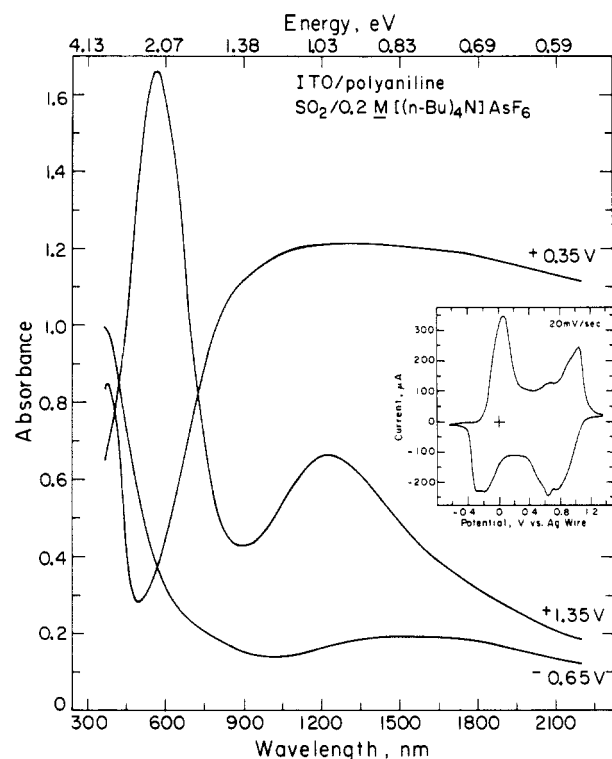
Figure 9. Visible-near-IR spectroelectrochemistry for polyaniline on ITO in \text{SO}_2/0.2 \text{ M } [(n\text{-Bu})_4\text{N}]\text{AsF}_6 at -70^\circ\text{C} . Inset: cyclic voltammetry of the same electrode in the spectroelectrochemical cell. Integration of the voltammogram indicates 3.4 \times 10^{-7} mol of repeat units per \text{cm}^2 of area covered by polymer.
