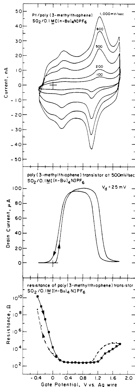
Figure 3. (Top) Cyclic voltammetry of II connecting three adjacent Pt microelectrodes in \text{SO}_2/0.1 \text{ M } [(n\text{-Bu})_4\text{N}]\text{PF}_6 at -40^\circ\text{C} . Integration of the voltammogram indicates reversible removal of 9 \times 10^{-8} mol of electrons per \text{cm}^2 of area covered by polymer. (Middle) I_D - V_G characteristic in the same medium for an adjacent pair of microelectrodes for which cyclic voltammetry is shown. Maximum conductivity on the positive sweep is \sim 10 \Omega^{-1} \text{ cm}^{-1} , and the window in which conductivity is at least 20% of maximum is 0.98 V wide. (Bottom) Steady-state resistance as a function of V_G for the same pair of microelectrodes for which the I_D - V_G characteristic is shown.
