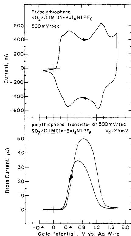
Figure 1. (Top) Cyclic voltammetry of I connecting three adjacent Pt microelectrodes in \text{SO}_2/0.1\ \text{M}\ [(n\text{-Bu})_4\text{N}]\text{PF}_6 at -40^\circ\text{C} . Integration of the voltammogram indicates reversible removal of 7 \times 10^{-7} mol of electrons per \text{cm}^2 of area covered by polymer. (Bottom) I_D – V_G characteristic in the same medium for an adjacent pair of microelectrodes connected with I for which cyclic voltammetry is shown. Maximum conductivity on the positive sweep is \sim 10^{-1}\ \Omega^{-1}\text{cm}^{-1} , and the window in which conductivity is at least 20% of maximum is 0.77 V wide.
