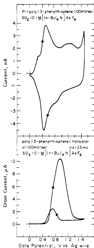
Figure 2. (Top) Cyclic voltammetry of III connecting two adjacent Pt microelectrodes in \text{SO}_2/0.1 \text{ M } [(n\text{-Bu})_4\text{N}]\text{AsF}_6 at -70^\circ\text{C} . Integration of the voltammogram indicates reversible removal of 1 \times 10^{-7} mol of electrons per \text{cm}^2 of area covered by polymer. (Bottom) I_D - V_G characteristic in the same medium for the same pair of derivatized microelectrodes. Maximum conductivity on the positive sweep is \sim 5 \times 10^{-2} \Omega^{-1} \text{ cm}^{-1} , and the window in which conductivity is at least 20% of maximum is 0.65 V wide.
