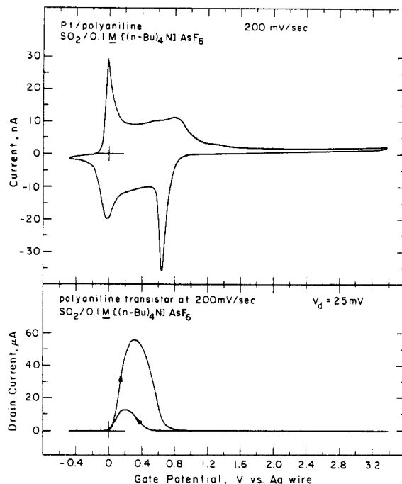
Figure 10. (Top) Cyclic voltammetry of polyaniline connecting two adjacent Pt microelectrodes in \text{SO}_2/0.1 \text{ M } [(n\text{-Bu})_4\text{N}]\text{AsF}_6 over activity I basic alumina at -70^\circ\text{C} . Integration of the voltammogram indicates 9.3 \times 10^{-8} mol of repeat units per \text{cm}^2 of area covered by polymer. (Middle) I_D - V_G characteristic in the same medium for the same pair of derivatized microelectrodes.
