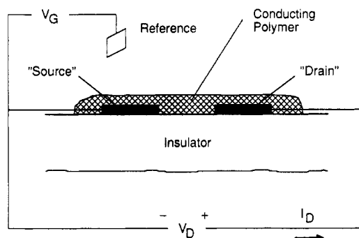
Scheme 1. Configuration of a Conducting Polymer-Based Transistor a
