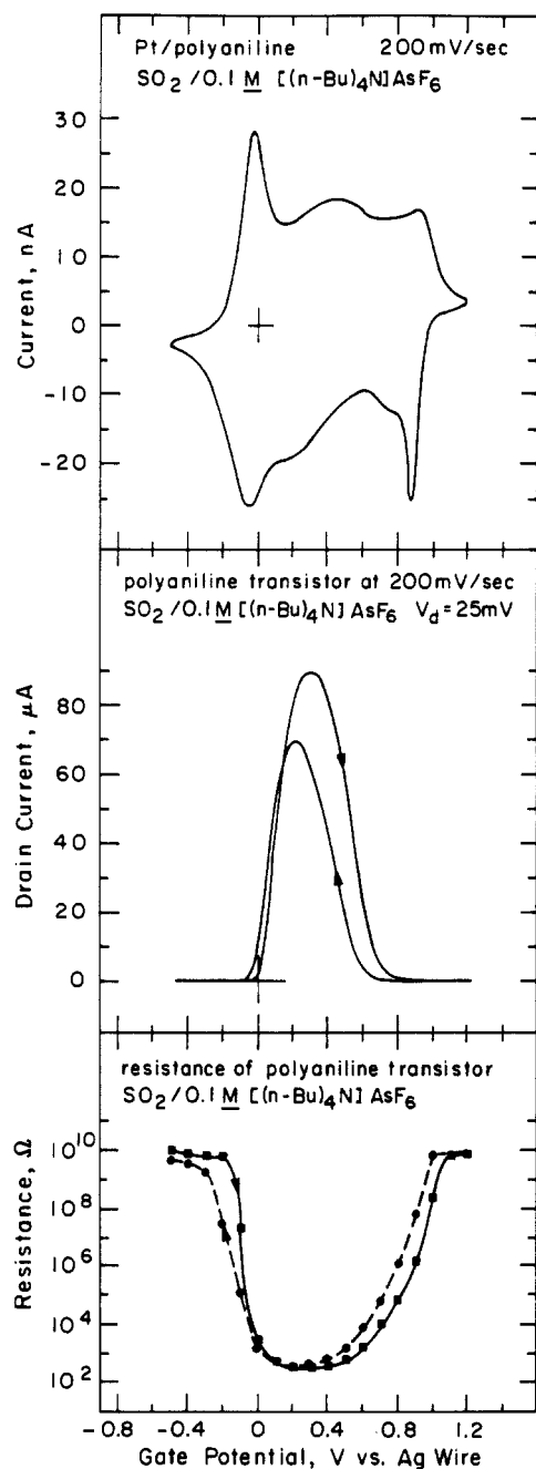
Figure 8. (Top) Cyclic voltammetry of polyaniline connecting two adjacent Pt microelectrodes in \text{SO}_2/0.1 \text{ M } [(n\text{-Bu})_4\text{N}]\text{AsF}_6 over activity I basic alumina at -70^\circ\text{C} . Integration of the voltammogram indicates 1.2 \times 10^{-7} mol of repeat units per \text{cm}^2 of area covered by polymer. (Middle) I_D - V_G characteristic in the same medium for the same pair of derivatized microelectrodes. Maximum conductivity on the positive sweep is \sim 1 \Omega^{-1} \text{cm}^{-1} , and the window in which conductivity is at least 20% of maximum is 0.6 V wide. (Bottom) Steady-state resistance as a function of V_G for the same pair of derivatized microelectrodes.
